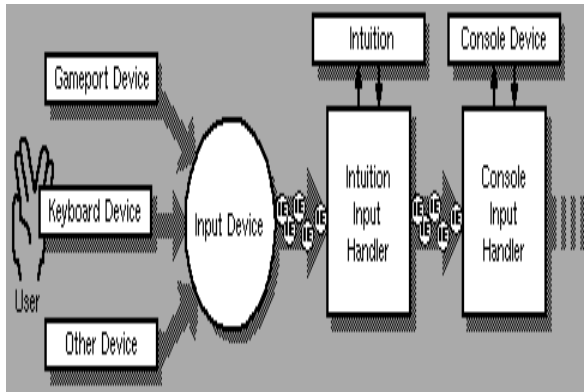
Figure 31-1: The Amiga Input Stream
