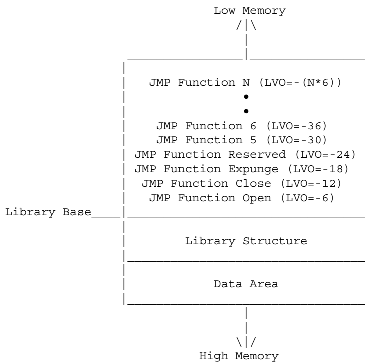
Figure 17-1: An Exec Library Base in RAM
