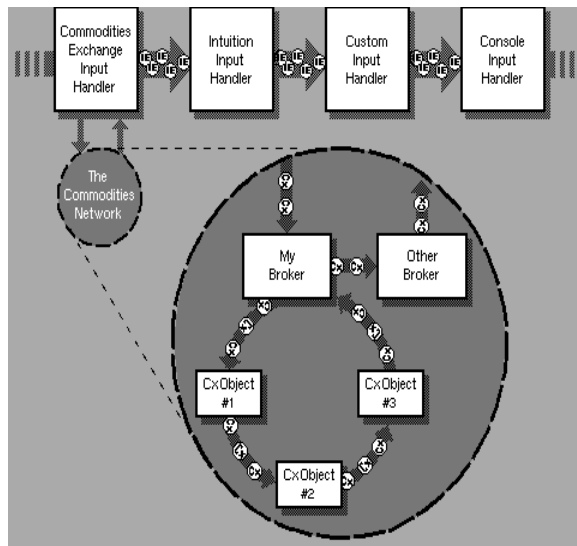
Figure 31-3: The Commodities Network
