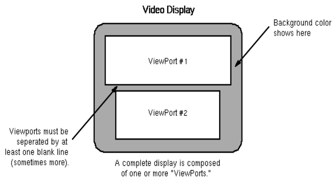
Figure 27-9: The Display Is Composed of ViewPorts
