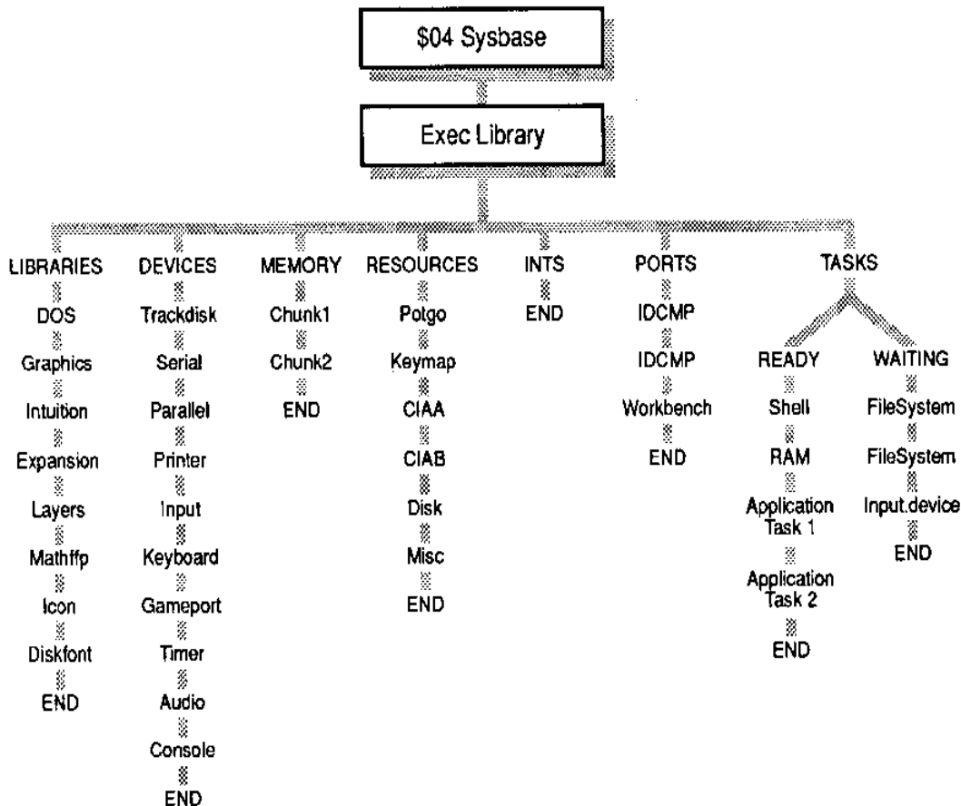
Figure 1-2: Exec and the Organization of the Amiga OS
