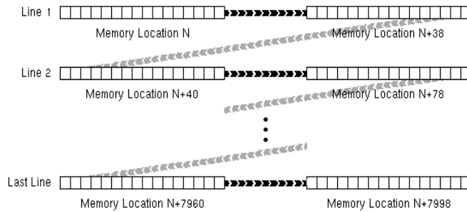
Figure 27-7: Bitplane for a Full-screen, Low-resolution Display
