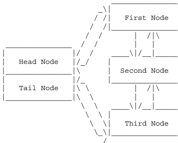
Figure 23-1: Simplified Overview of an Exec List
