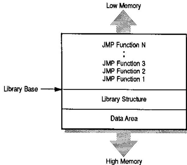
Figure 1-1: Amiga Library Structure and Jump Table
