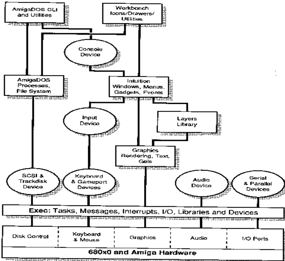
Figure 1-1: Amiga System Software Hierarchy
