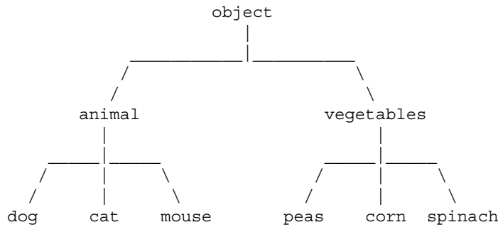
Figure 12-1: Object Diagram
