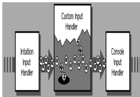
Figure 31-2: A Custom Input Handler
