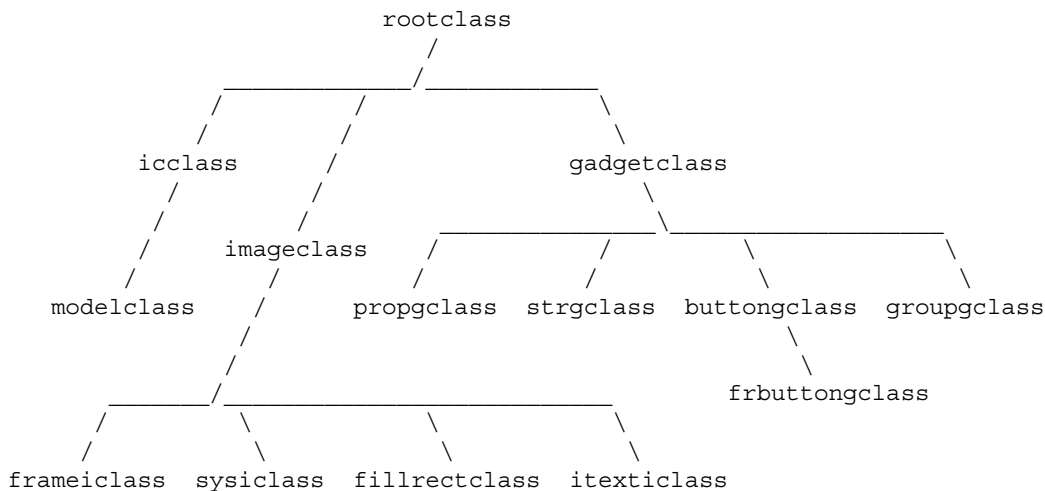
Figure 12-3: Class Diagram
