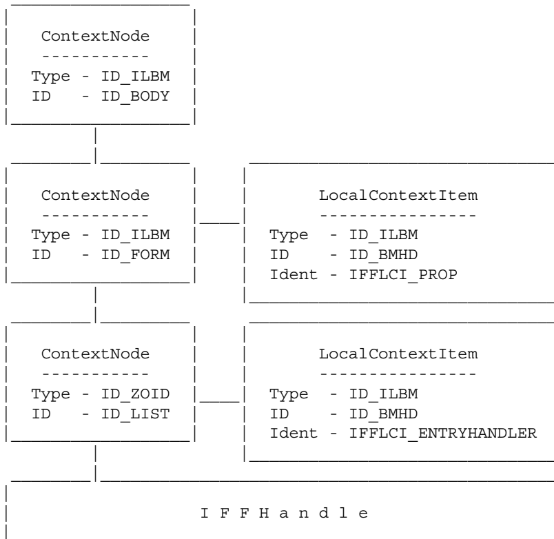
Figure 33-3: IFFParse Context Stack
